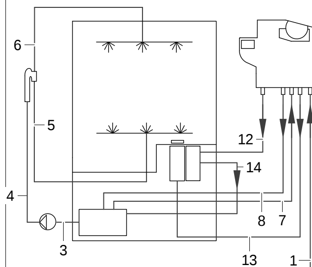
Water softener
